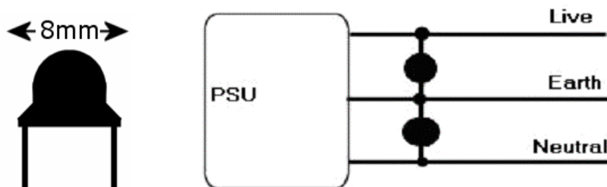
(a) Appearance and dimensions of PSU suppressor and (b) connection to PSU
