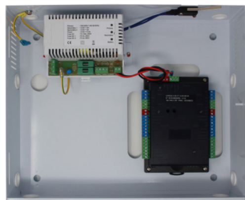
Figure 1: 4 Door Controller + Metal Case + 5A PSU
